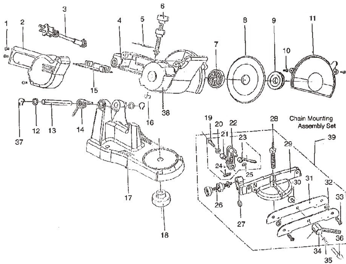
Assembly Drawing
