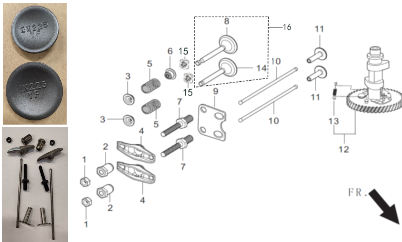
FIG.5 TRAIN,VALVE / CAMSHAFT SUBASSEMBLY (E05)
