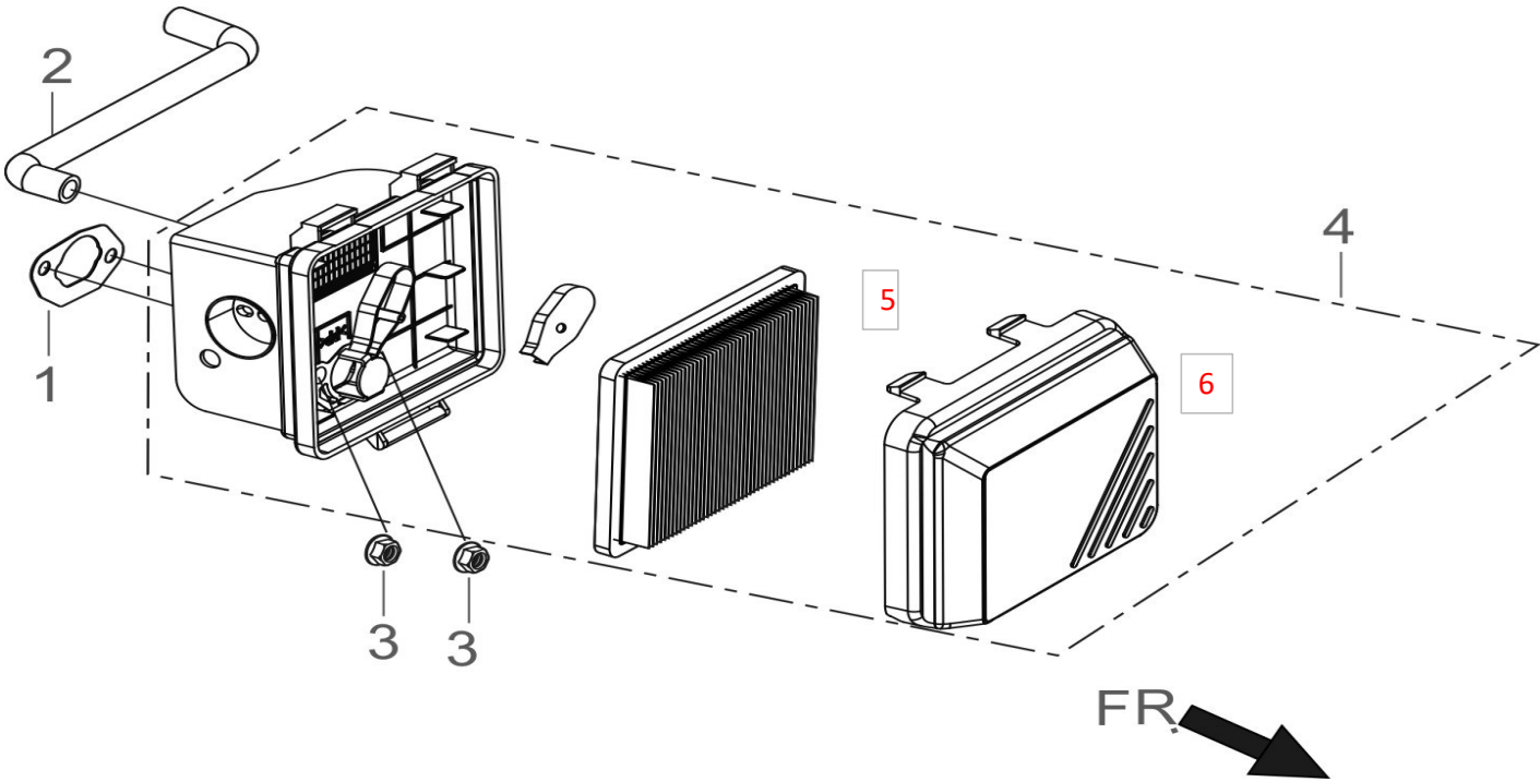
FIG.11 CLEANER, AIR (F01)
