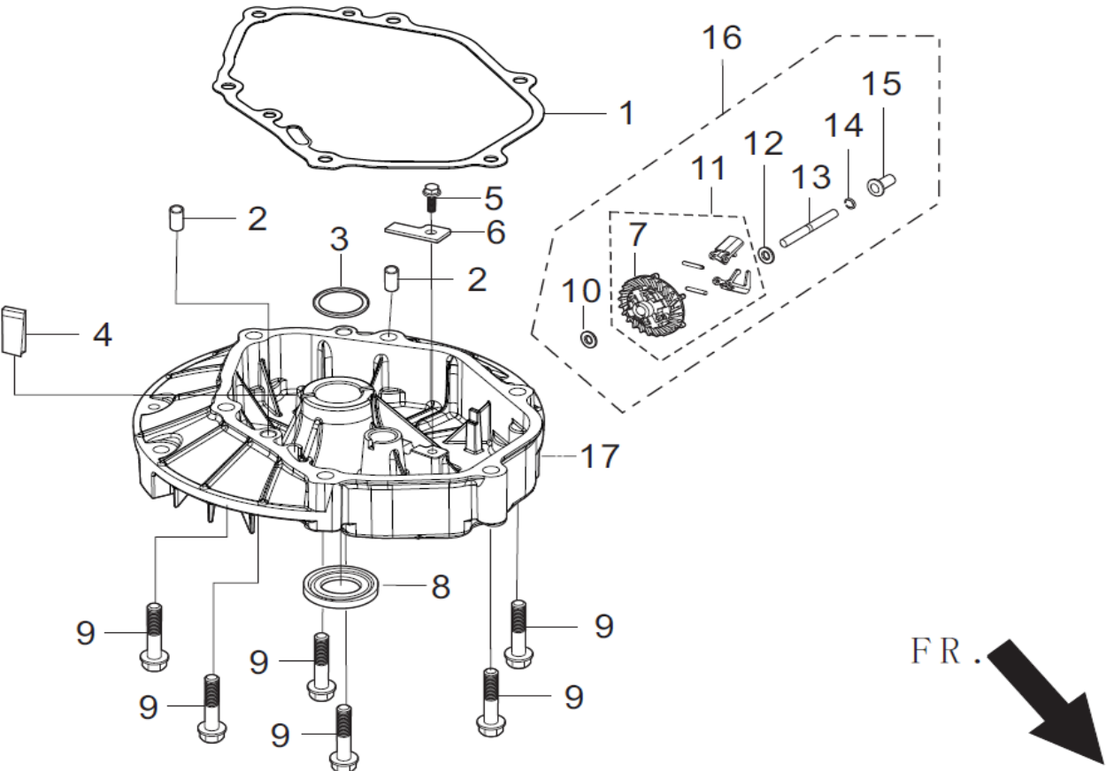
FIG.2 COVER SUBASSEMBLY, CRANKCASE / GEAR ASSY, GOVERNOR (E02)
