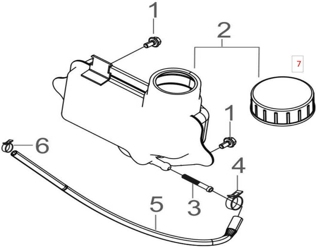
FIG.13 TANK, FUEL (F03)
