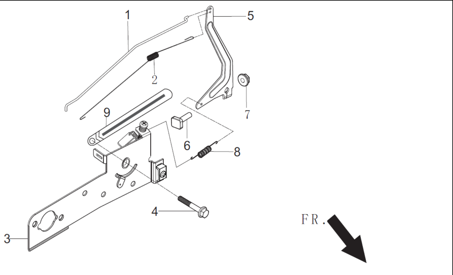
FIG.10 CONTROL ASSY, THROTTLE (E10)
