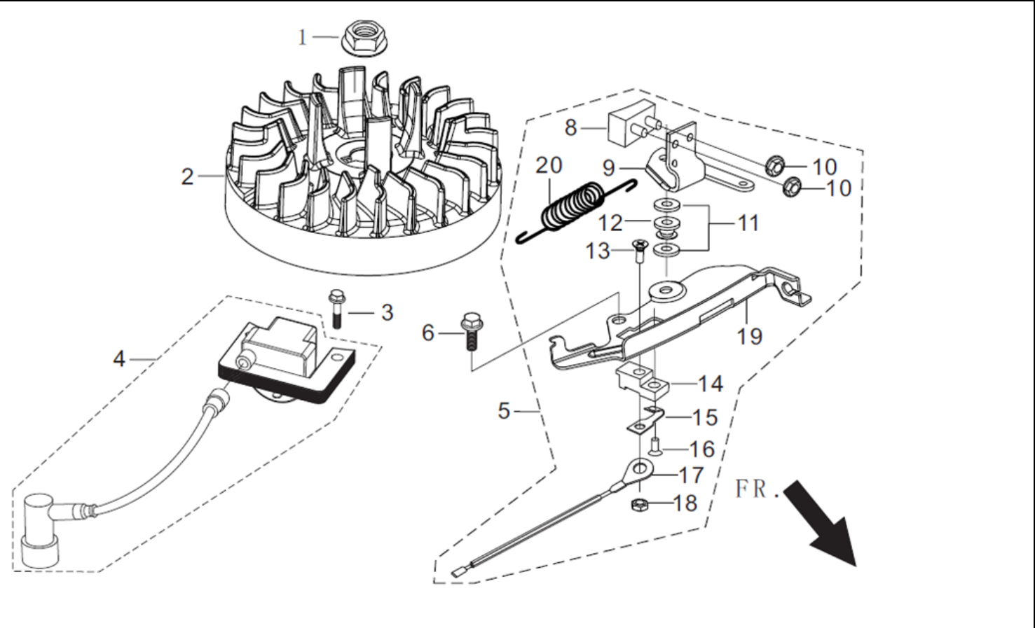
FIG.9 FLYWHEEL / IMPELLER / STARTER PULLEY / IGNITION COIL (E09)
