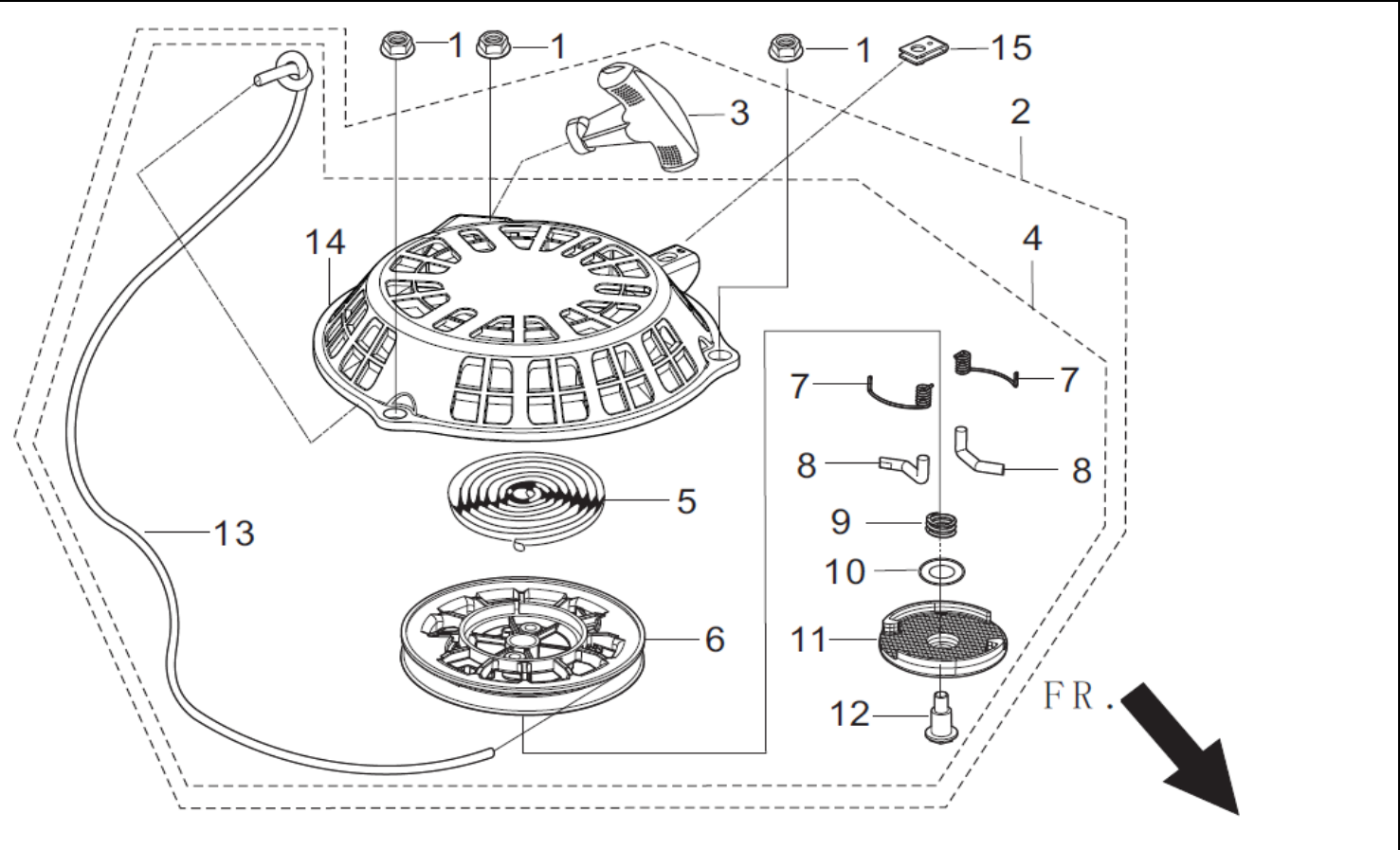
FIG.6 STARTER,RECOIL (E06)
