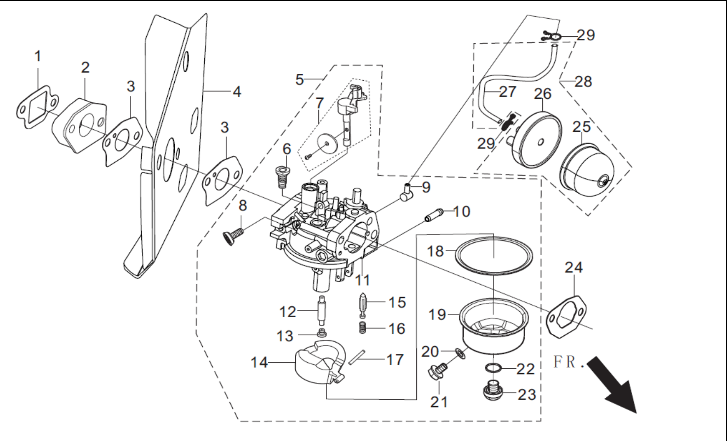
FIG.8 CARBURETOR ASSY. (E08)
