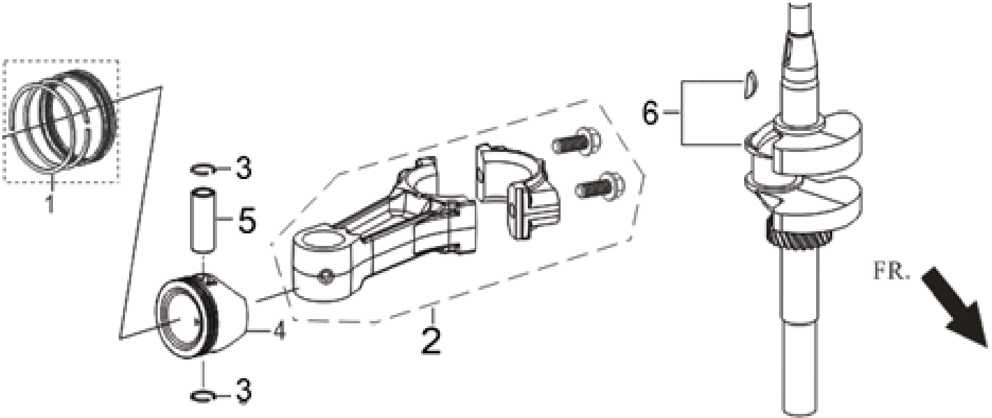
FIG.4 ROD,CRANKSHAFT CONNETING (E04)
