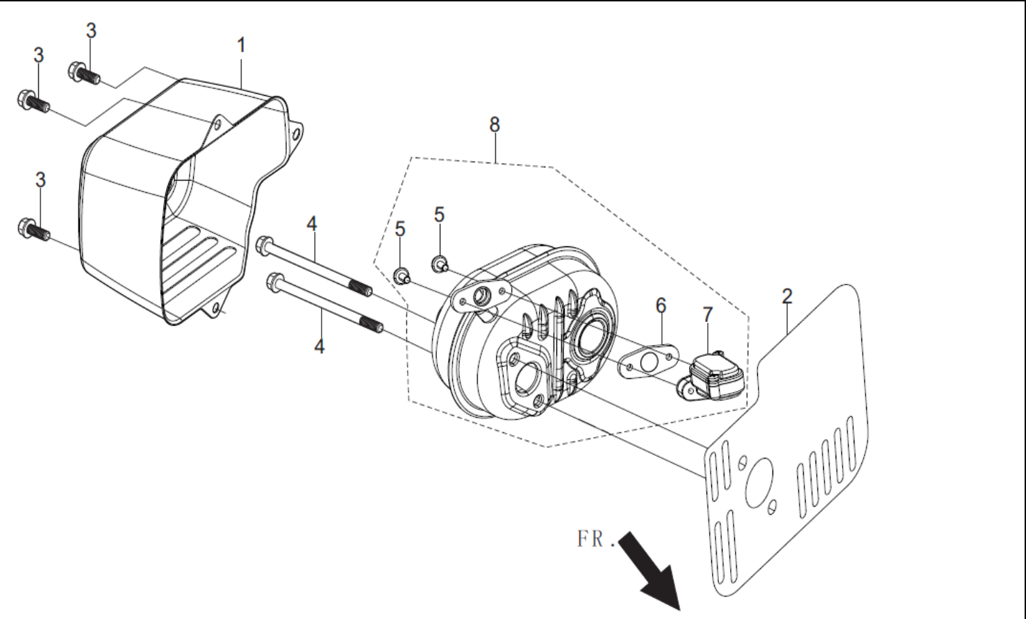
FIG.12 MUFFLER (F02)
