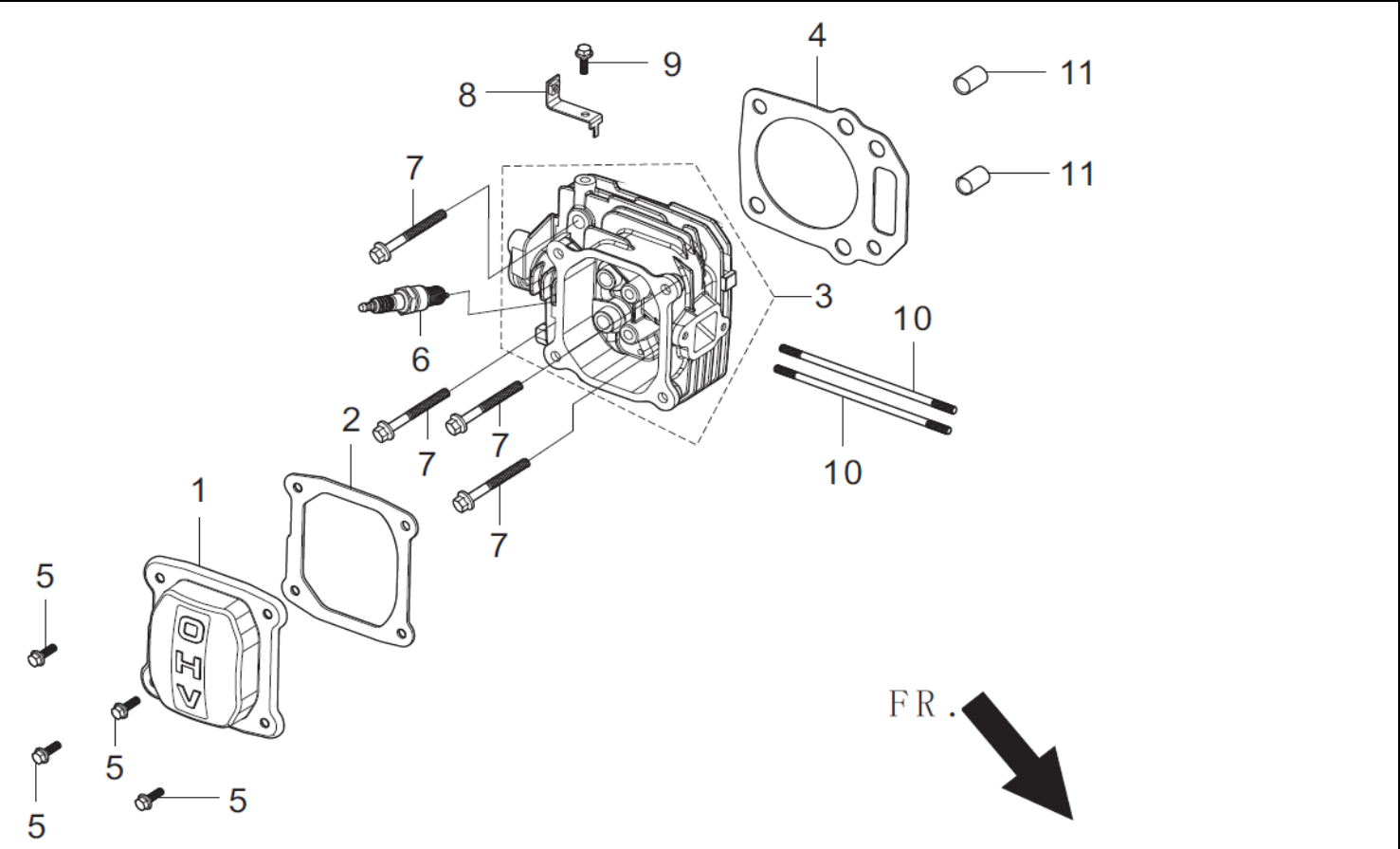
FIG.3 HEAD SUBASSEMBLY, CYLINDER / PLUG,SPARK (E03)
